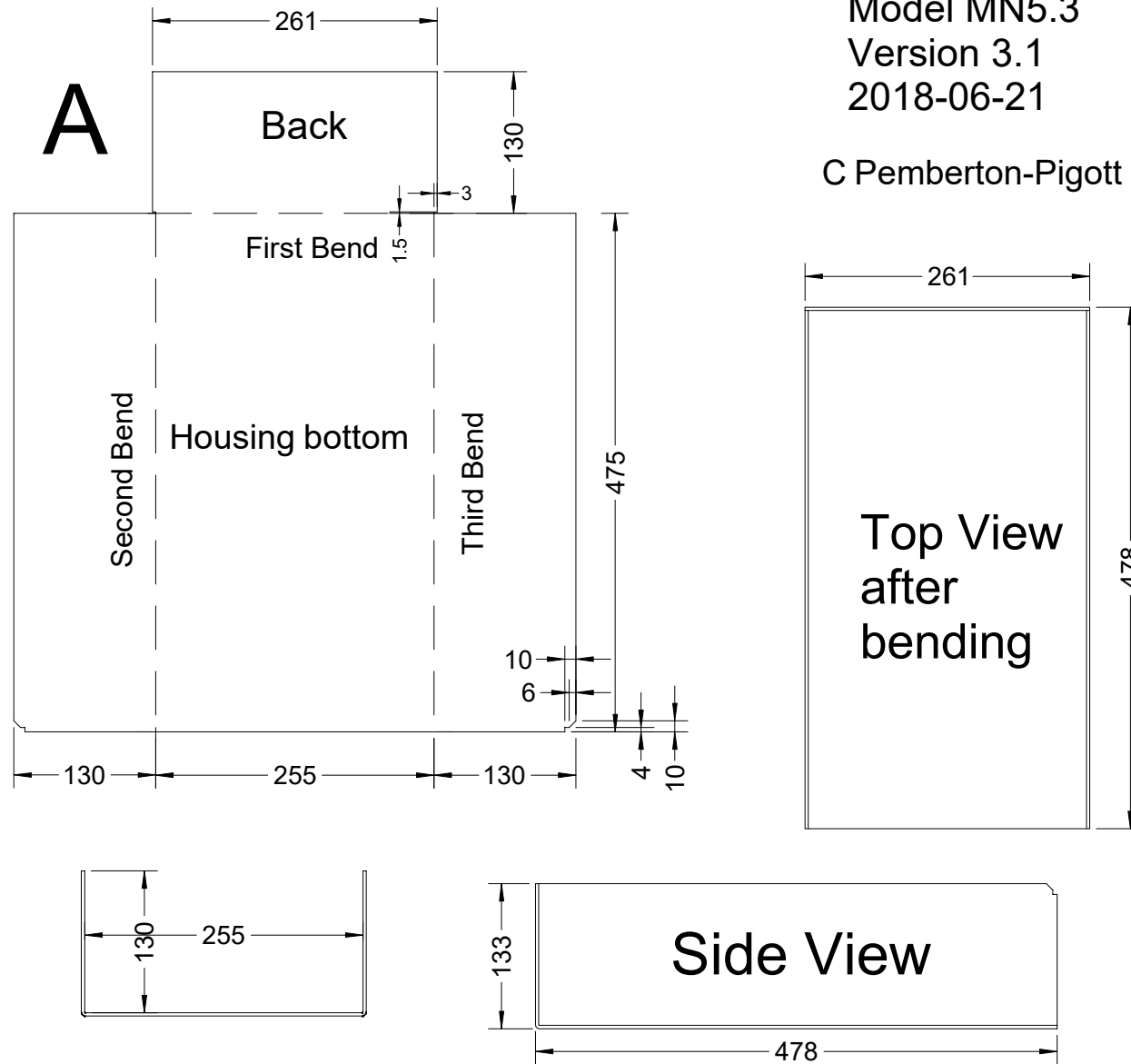
Front Ash Drawer Housing
